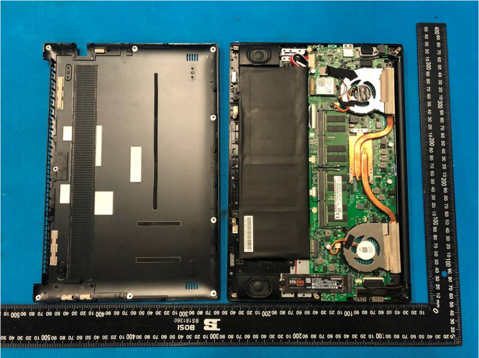
Photo 7: Internal view
